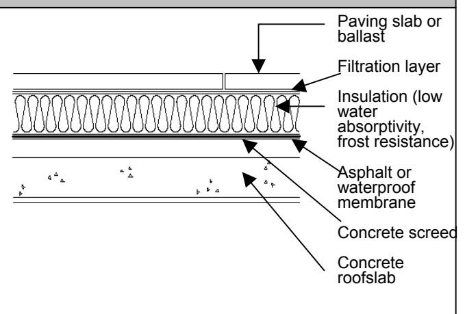
Diagram B7 Para. B.5.5 Inverted warm deck roof with concrete structure
