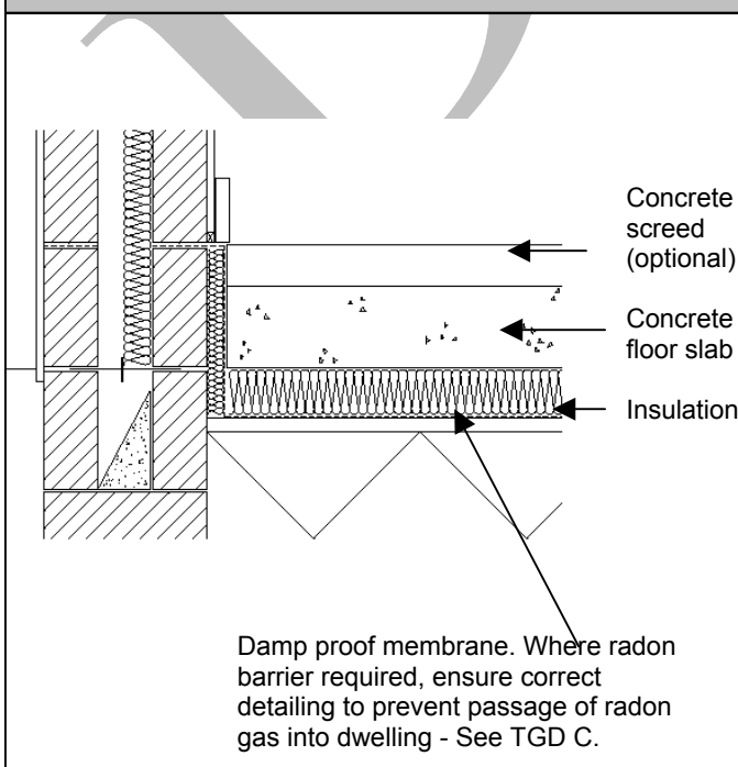
Diagram B12 Para. B.7.1 Concrete slab-on-ground floor, insulation under slab
