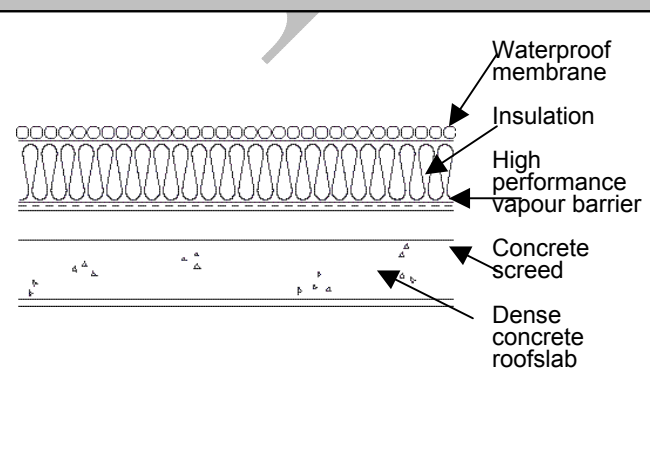
Diagram B6 Para. B.5.4 Sandwich warm deck flat roof above a concrete structure
