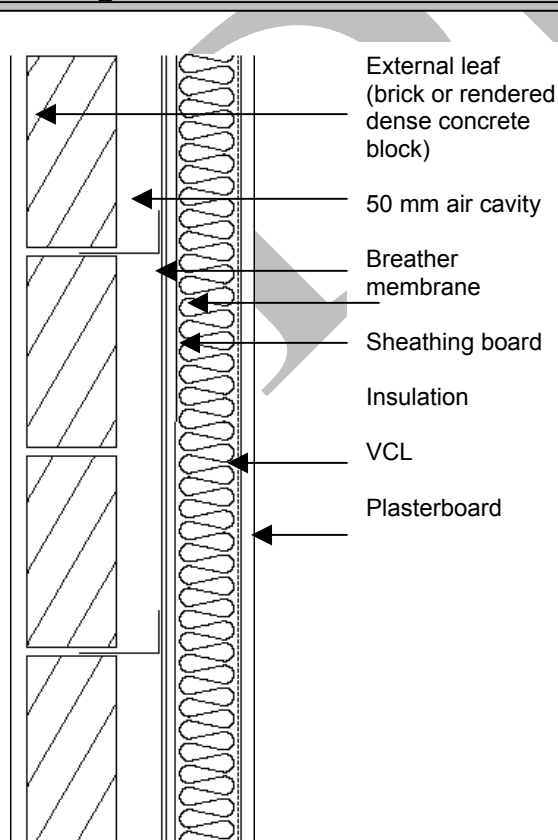
Diagram B10 Para. B.6.3.1 Timber frame wall, insulation between framing timbers.
