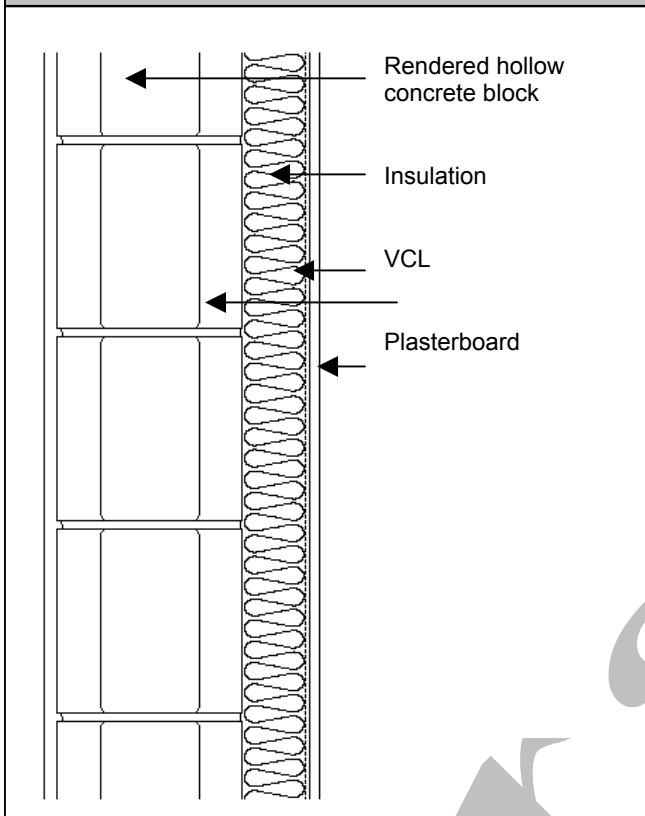
Diagram B11 Para. B.6.4 Hollow-block wall, internal insulation lining
