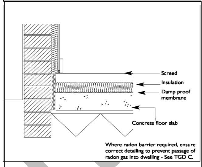
Diagram B13 Para. B.7.1 Concrete slab on ground floor, insulation under screed
