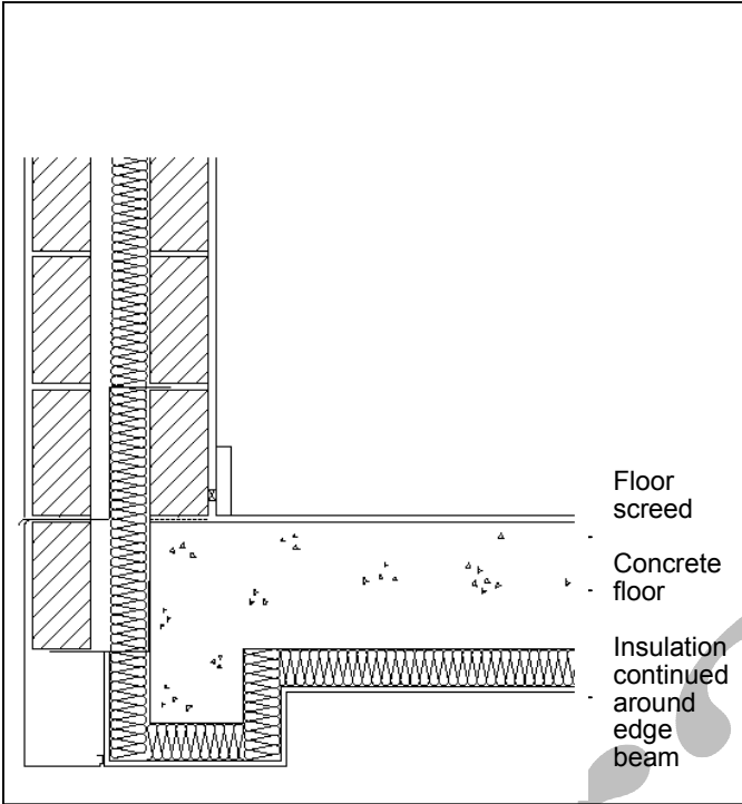
Diagram B19 Para. B.7.5 Exposed concrete floor, external insulation
