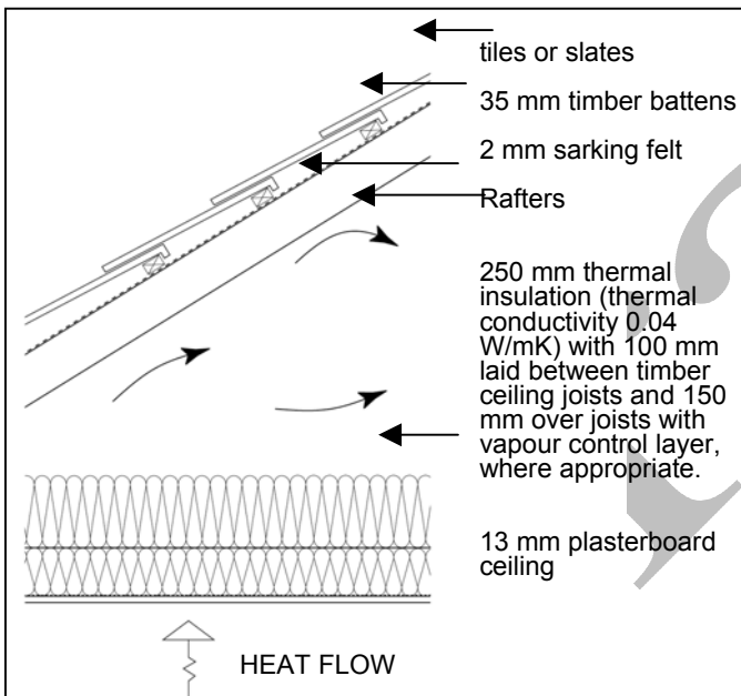
Diagram A3 Para. A.2.2 Domestic pitched roof
